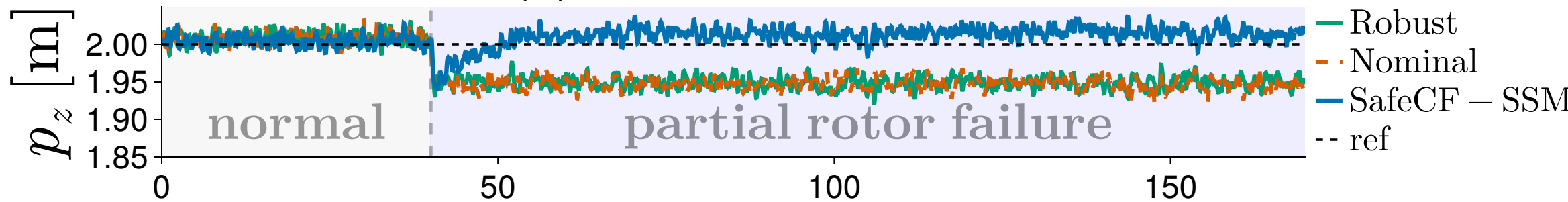
(a) Altitude Tracking
