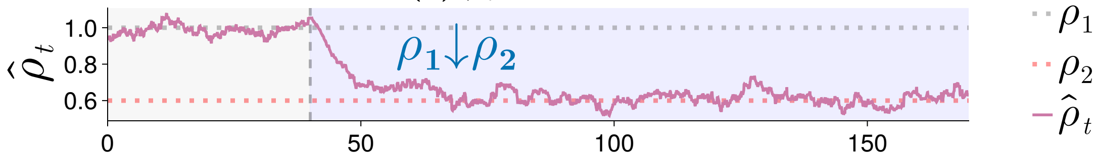
(c) \hat{\rho}_t adaptation
